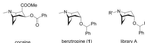
Fig. 1 Cocaine, benztropine and the target library.
