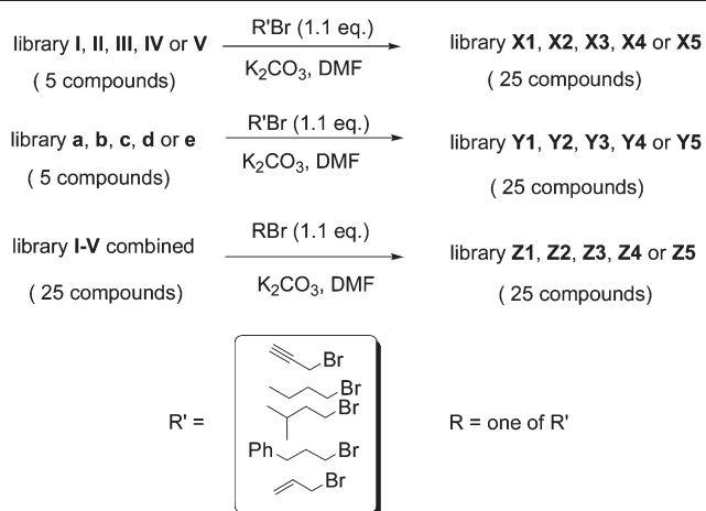
Scheme 5 Synthesis of libraries X_1 to Z_5 .
