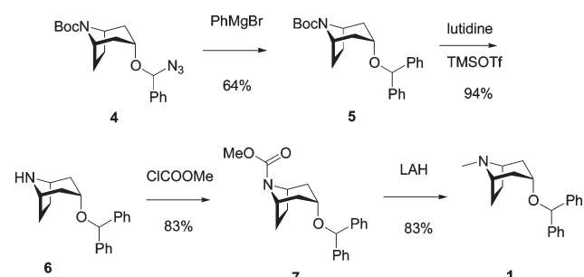
Scheme 2 Synthesis of benzotropine from the azidoether 4 .
